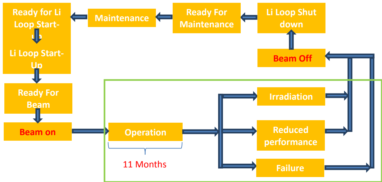
Fig. 1. General scheme of IFMIF operation
