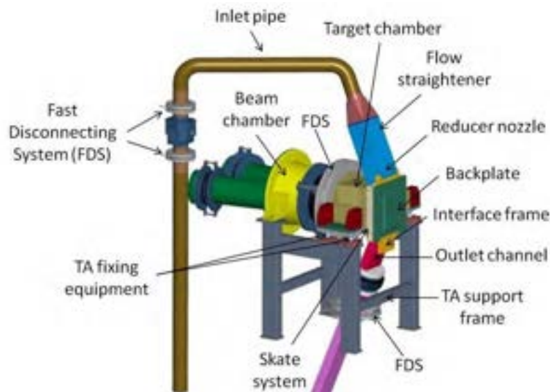
Fig. 2. The EU target system
