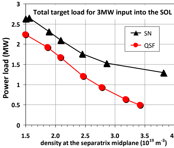
Figure 4. Total load on both targets versus the plasma density at the outboard midplane. The power input into the SOL is 3.0 MW.
