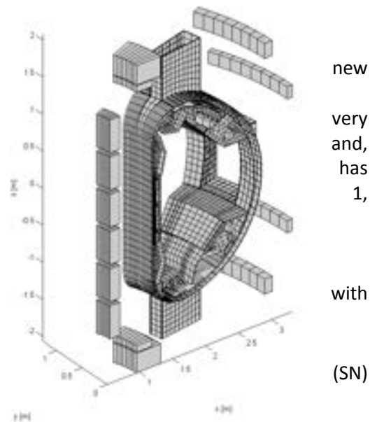
Figure 2. Details of the 3D mesh used for vertical stability analyses. [11].
