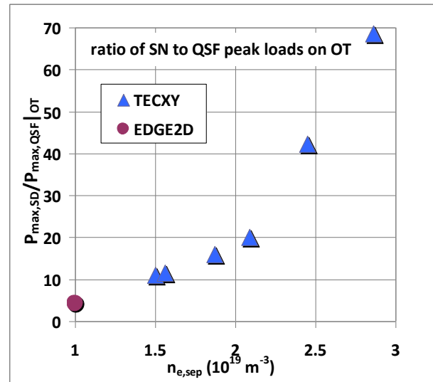
Figure 6. QSF peak mitigation factor, as derived from TECXY and EDGE2D runs. The point from this last code aligns very well to the others, despite the very different calculation method.
