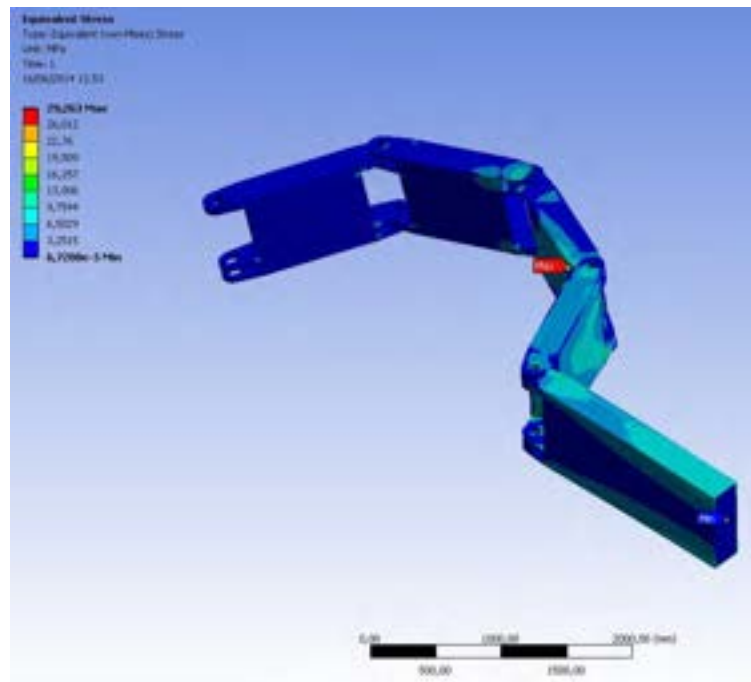
Figure 5 - Stress in the robot arm
