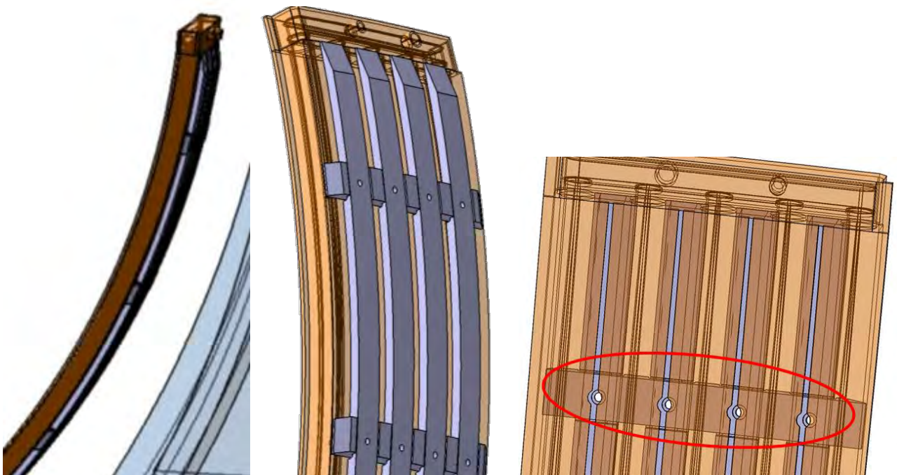
Fig. 4 - Ribs design
