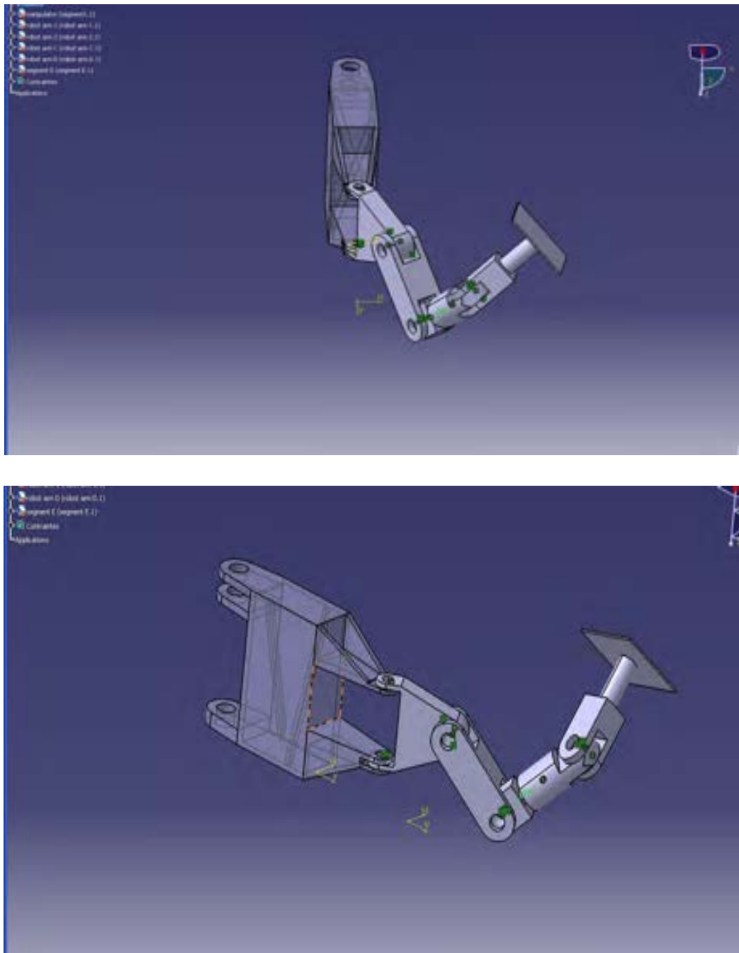
Figure 7 - Last segment handling robot
