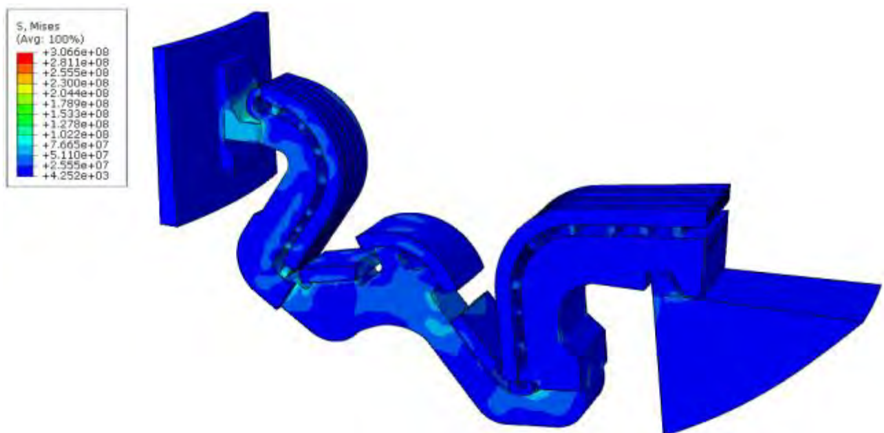
Fig. 25. Von Mises Stresses overview: time instant 67.9ms.
