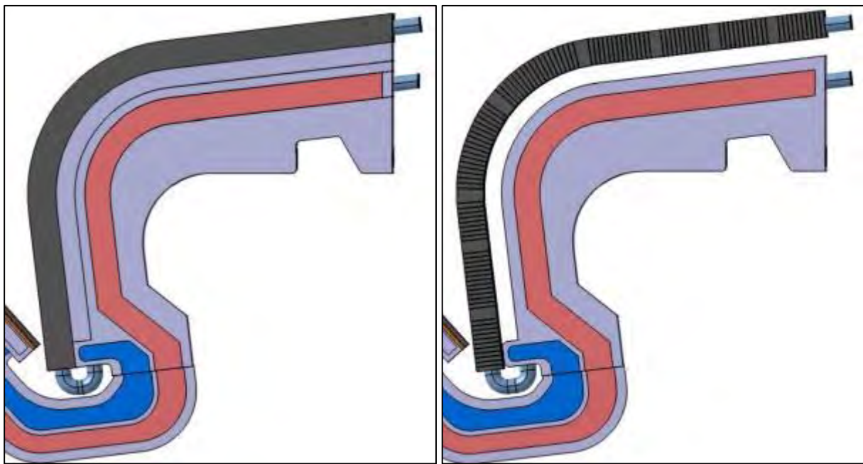
Fig. 10 Outer vertical target side
