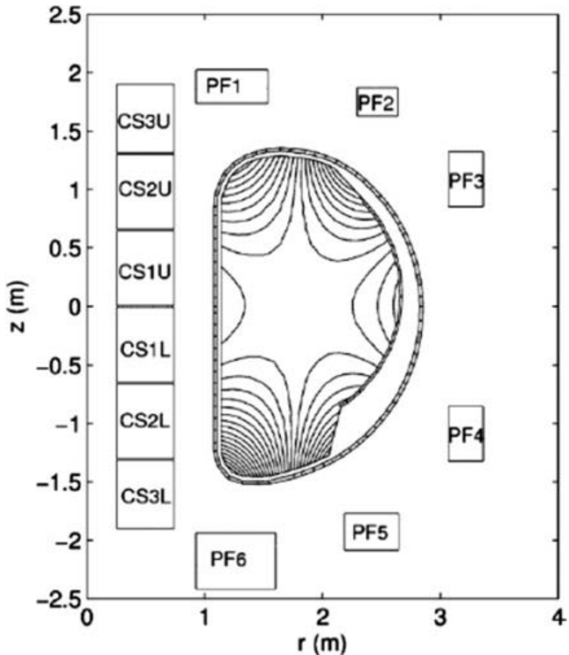
Figure 5. Simplified sketch of the FAST magnetic system (TF coil is not shown)
