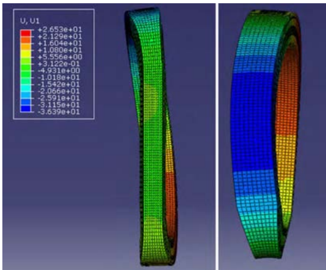
Figure 4. TF 3D ABAQUS analysis with the deformations magnified to be more evident
