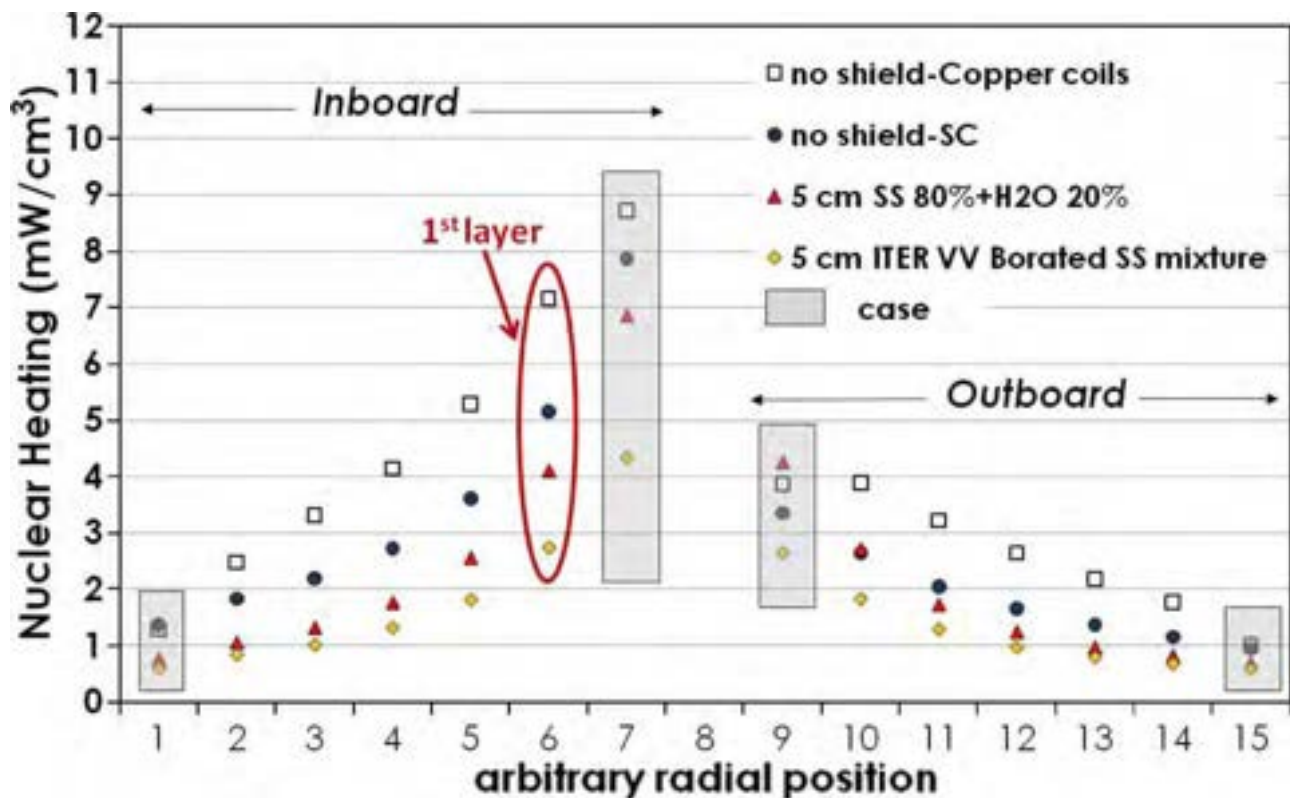
Figure 1. TF NH radial profile used to investigate the effect of the presence of a nuclear shield
