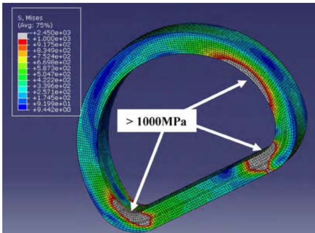
Figure 3. TF 3D ABAQUS analysis with the areas where Von Mises stress is higher than 1000 MPa evidenced
