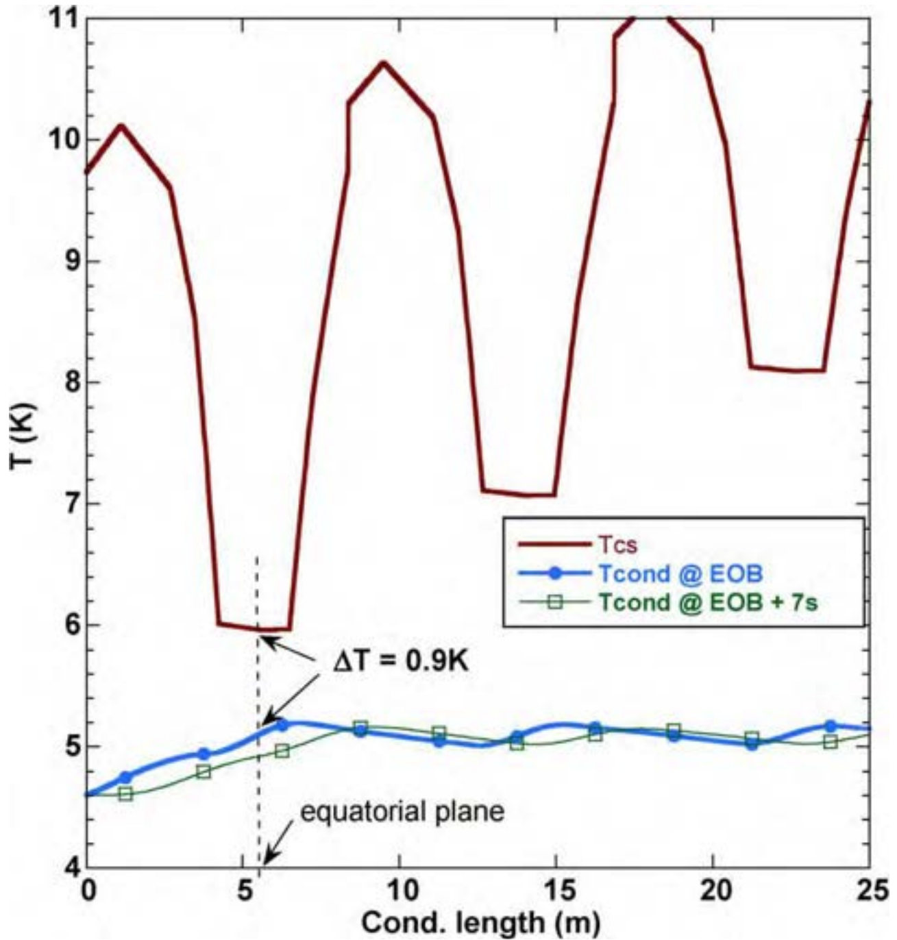
Figure 2. TF conductor temperature analysis with a minimum temperature margin of 0.9 K found at the equatorial plane, innermost layer at the inboard leg
