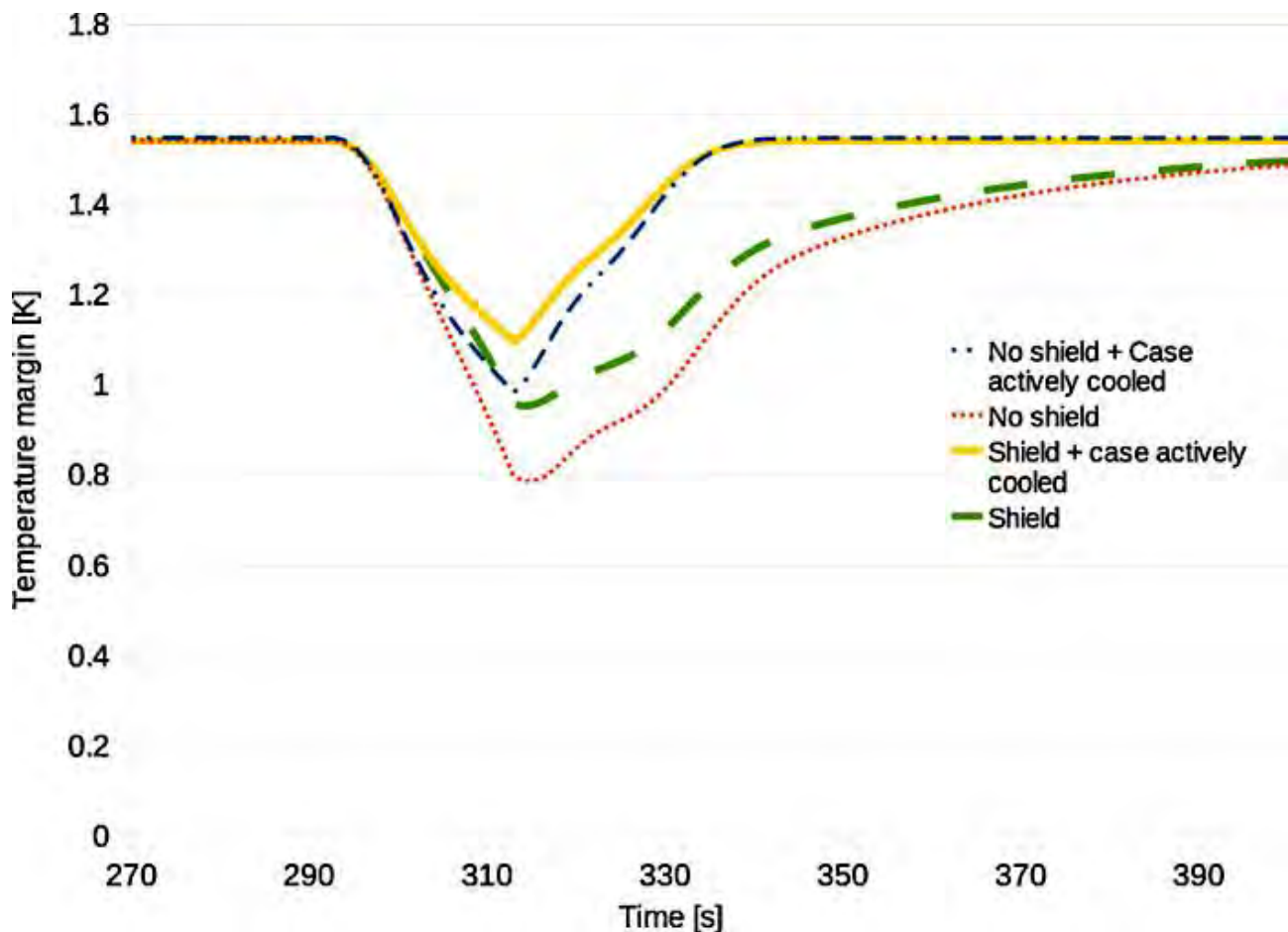
Figure 9. Temperature margin evolution in the most critical location (equatorial plane) in the four cases
