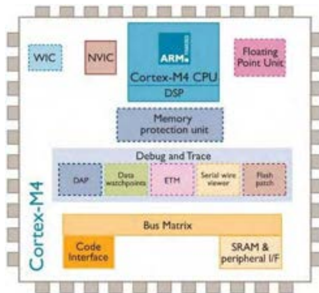
Figura 13: Cortex-M4 implementation
