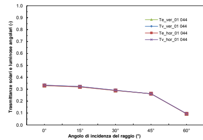
01044 – Tessuto in PET nero con coating in Cr
