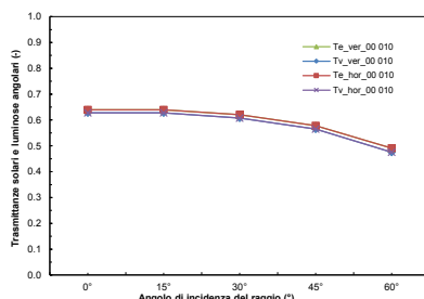
00010 – Tela metallica in rame
