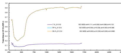
01012 – Tessuto in PVDF a maglia larga
