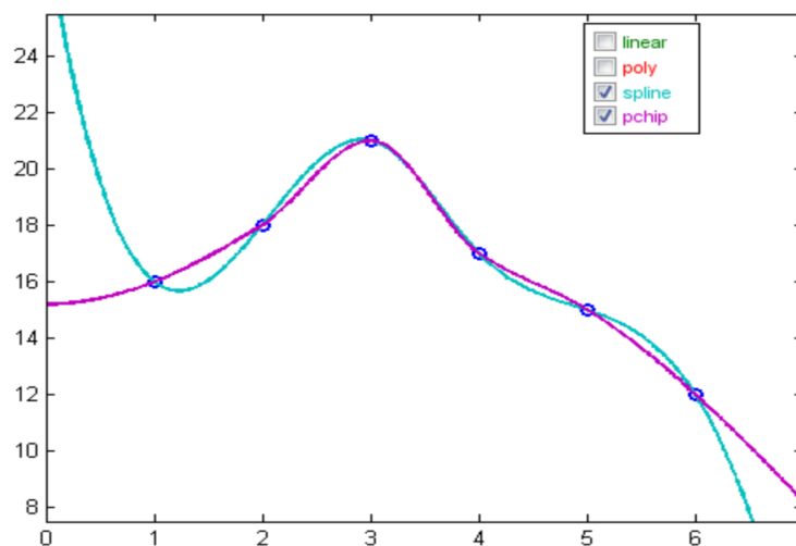
Figura 7 – Fonte: https://blogs.mathworks.com/cleve/2012/07/16/splines-and-pchips/
