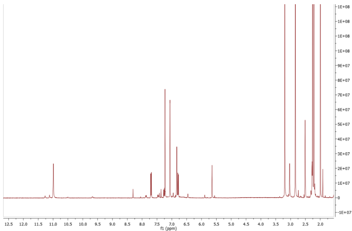
Figura 12. ^1\text{H} NMR spectrum ( \text{DMSO}-d_6 ) of compound 3f .
