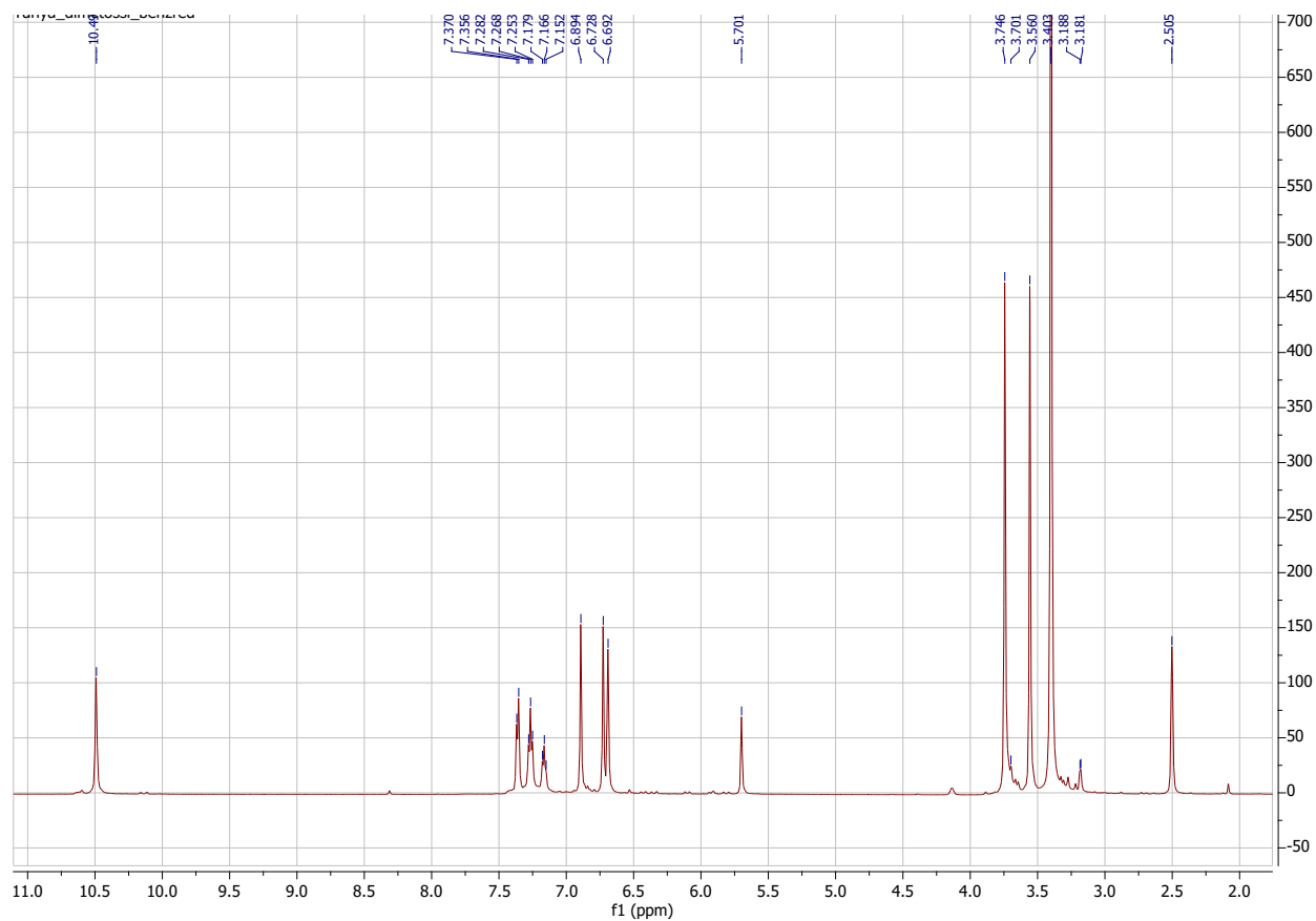
Figura 6. ^1\text{H} NMR spectrum ( \text{DMSO}-d_6 ) of compound 3a.
