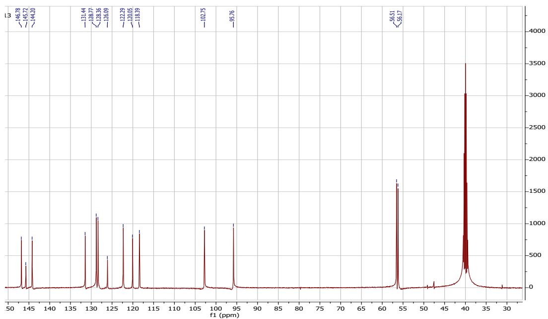
Figura 7. ^{13}\text{C} NMR spectrum ( \text{DMSO}-d_6 ) of compound 3a.
