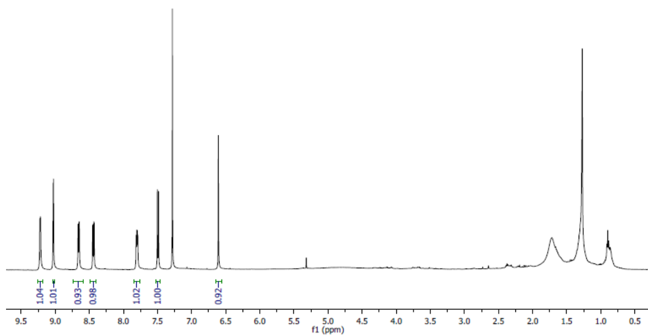
Figura 38. ^1\text{H} NMR spectrum ( \text{CDCl}_3 ) of compound 5c.
