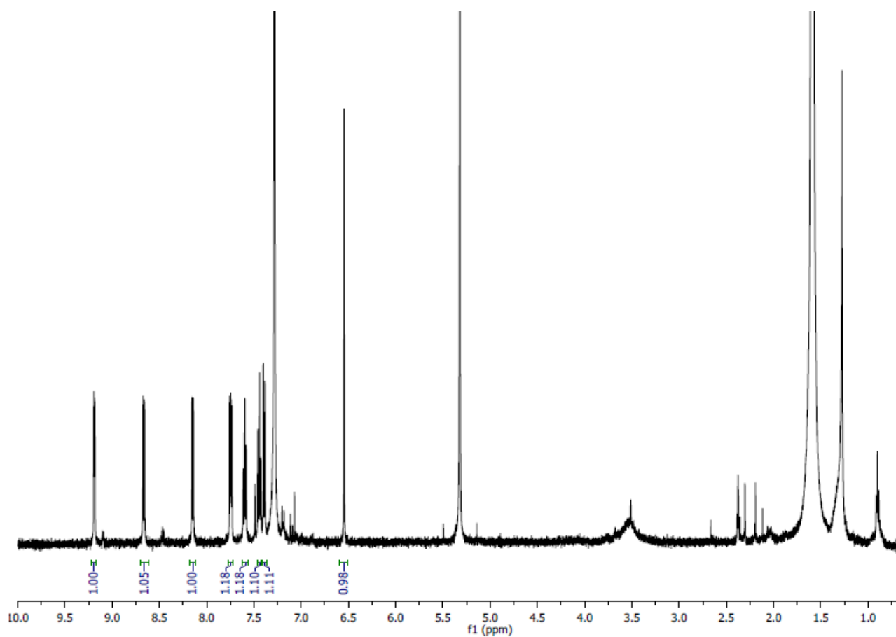
Figura 35. ^1\text{H} NMR spectrum ( \text{CDCl}_3 ) of compound 5a.
