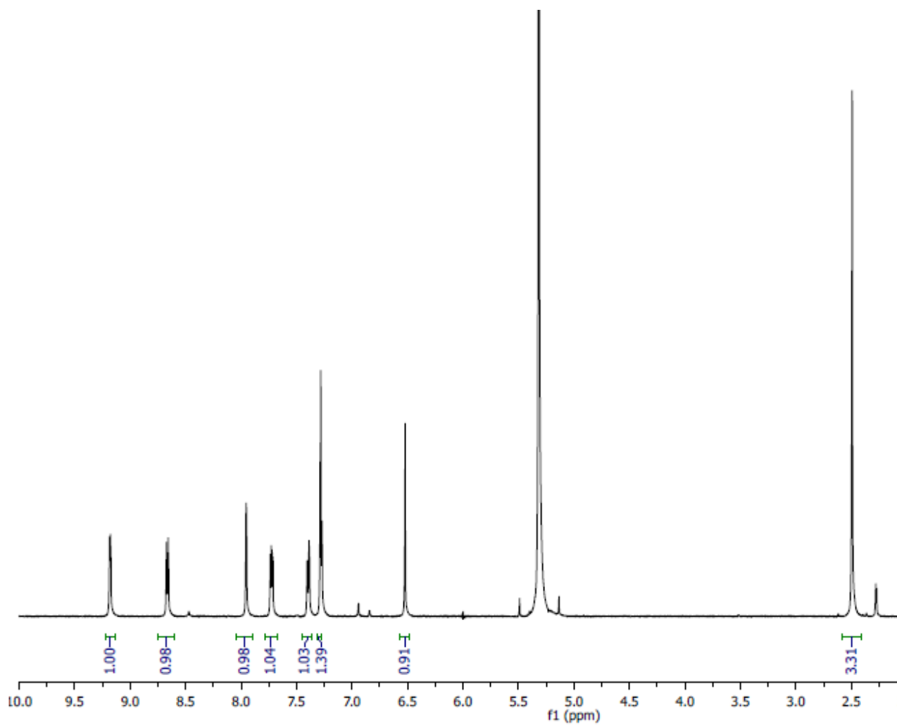
Figura 36. ^1\text{H} NMR spectrum ( \text{CDCl}_3 ) of compound 5b.
