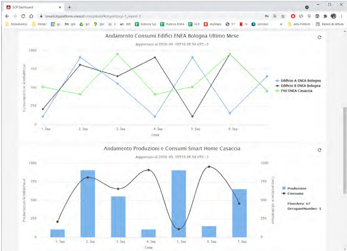
Figura 24 - SCP-DASH Report Screenshot 3
