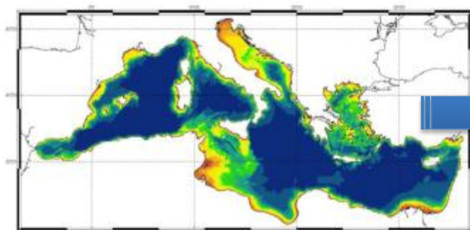
WAM (1/16° x 1/16° )
