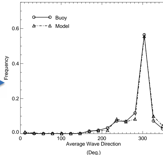
Frequency distribution of model and buoy average wave direction at Alghero . Only records with H_s > 1 m are considered. Incoming wave direction is indicated as degrees in clockwise direction from the north.
