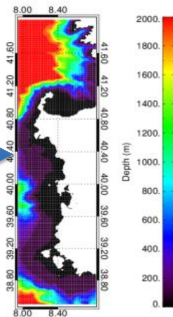
WAM/SWAN (1/120° x 1/120° )
