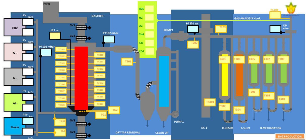
GESSICA an experimental plant for studies about Gasification, SNG and P2G
